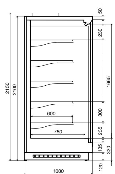
Vega DG 100 H210
