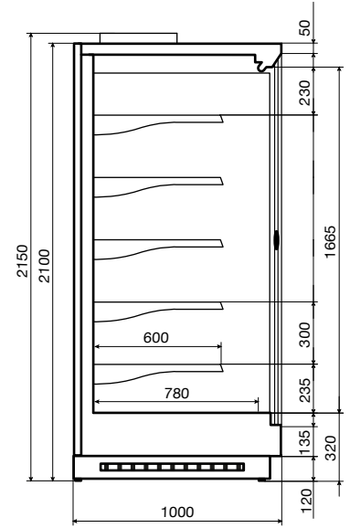
Vega SG 100 H210
